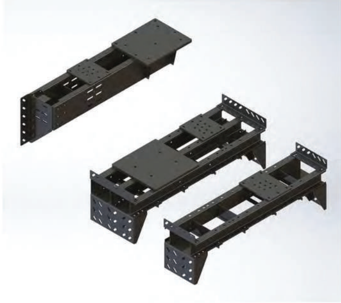
MRL 2:1 makine sehpaları, raya montaj / duvara montaj MRL 2:1 machine frames, rail mounting / wall mounting
